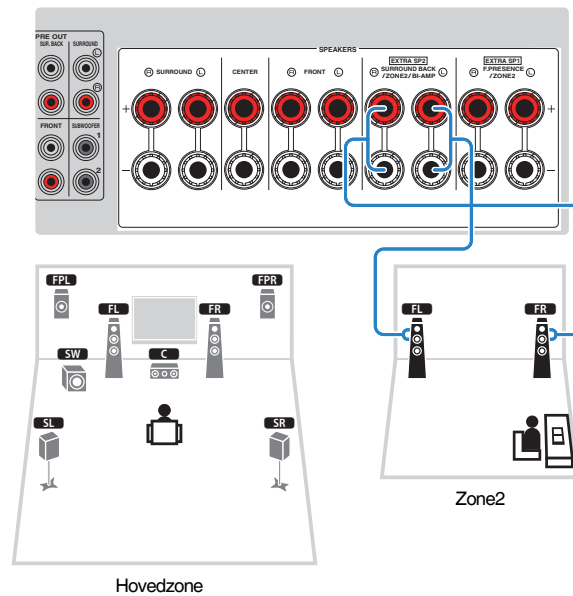
Enheden (bagside)
