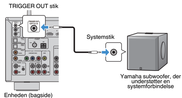
Enheden (bagside)
