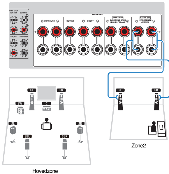
Enheden (bagside)
