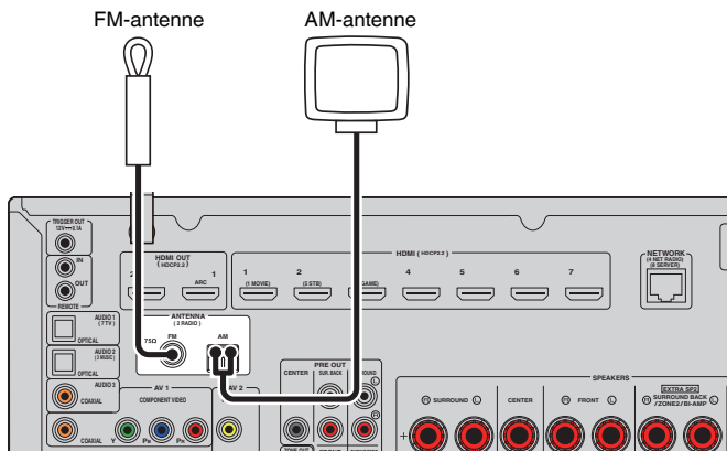
Enheden (bagside)
