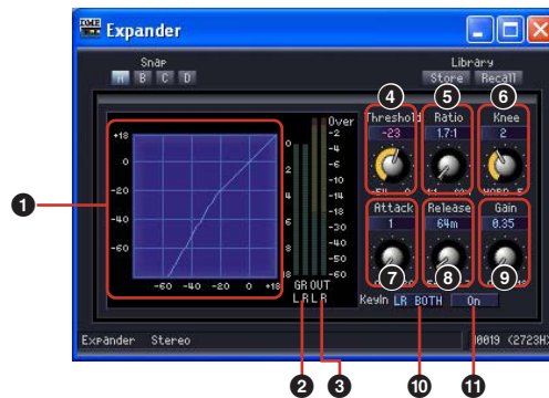
Expander component editor
