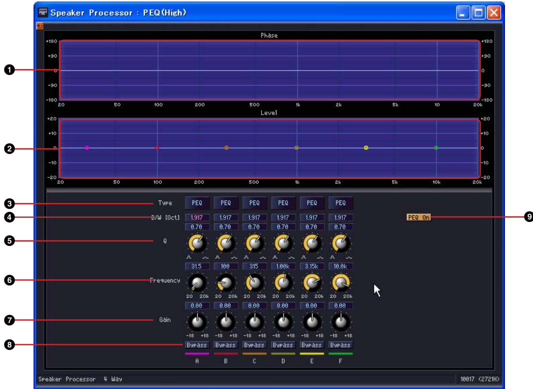
[Speaker Processor - PEQ] edit window
