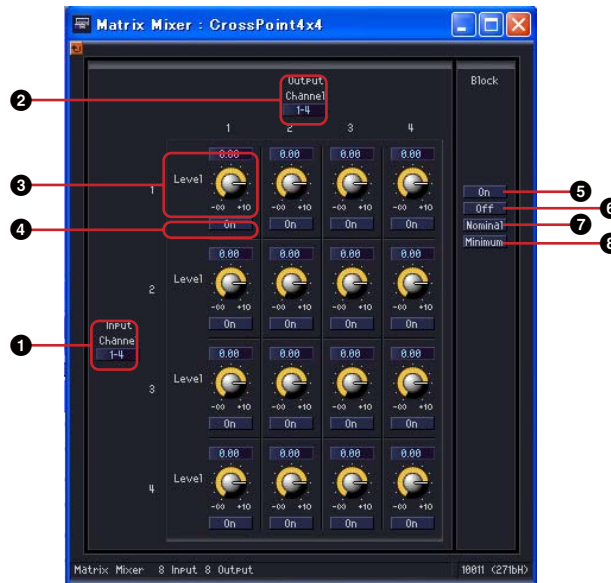
[Matrix Mixer - Crosspoint] editor window
