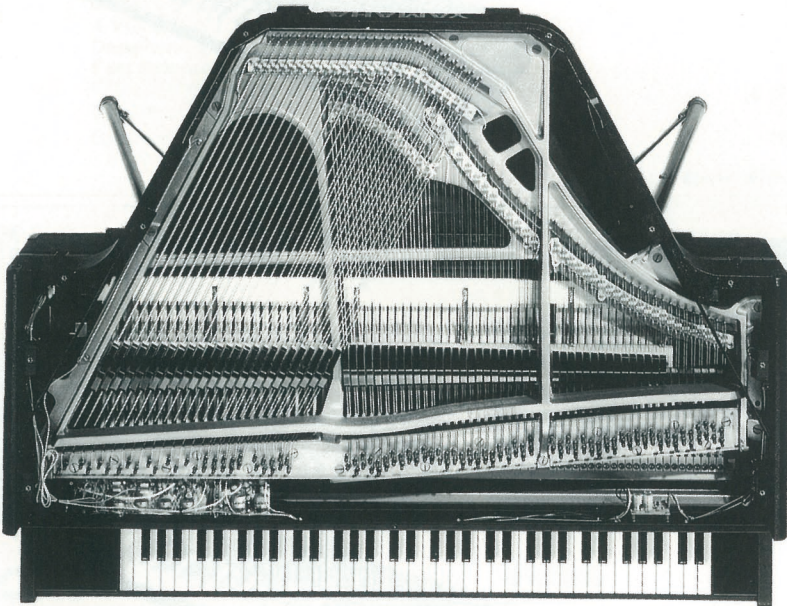
CP70B 73 keys (E 0 ~ E 6 ) Controls: Bass, Middle, Treble, Tremolo Speed and Depth, Volume
