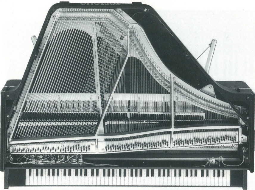
CP80 88 keys (A-1 ~ C7) Controls: Bass, Middle, Treble, Brilliance Level Selector Switch, Tremolo Speed and Depth, Volume
